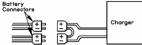
Figure 10-2 Series Charging Connections
