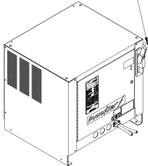
Figure 10-3 Fused Disconnect Switch
