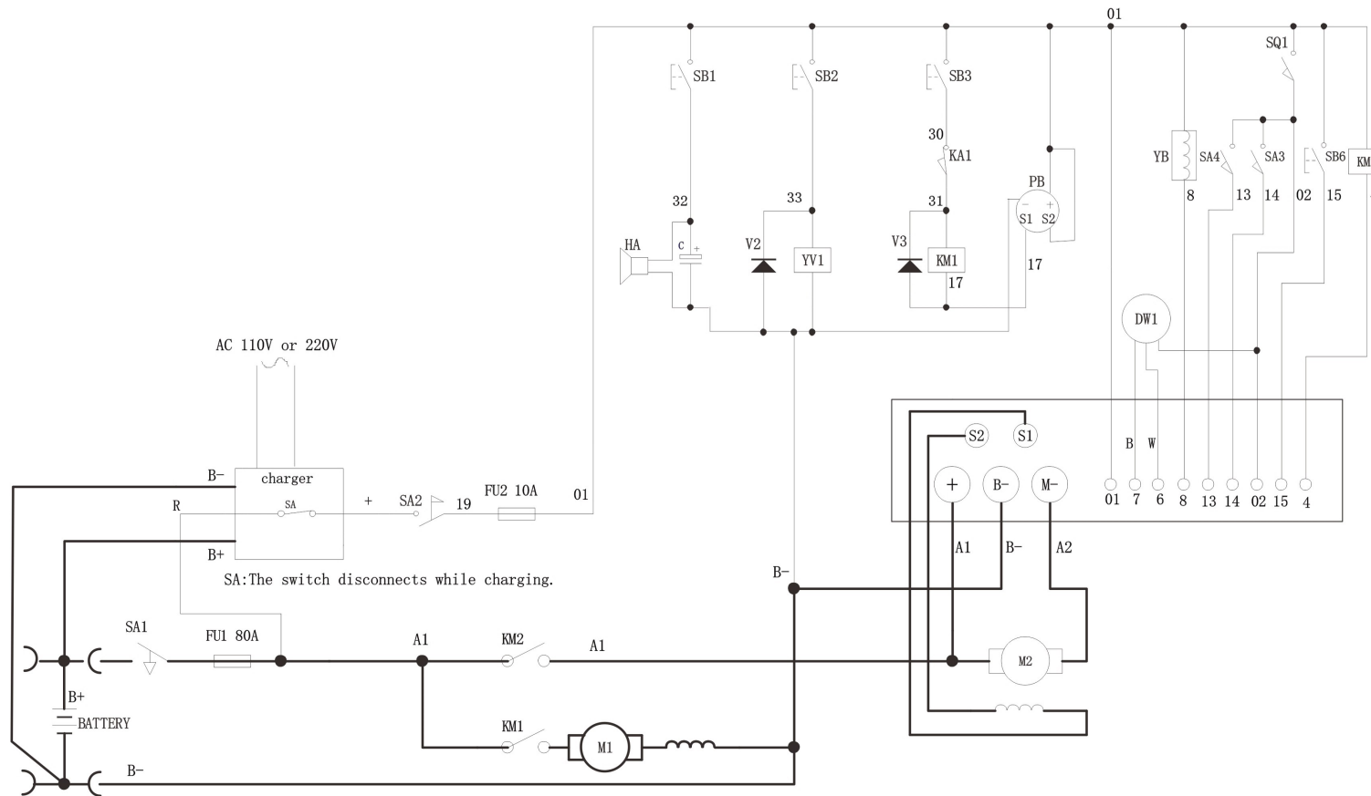
Title:170G/610/050/070/080/090/070E electric system diagram
